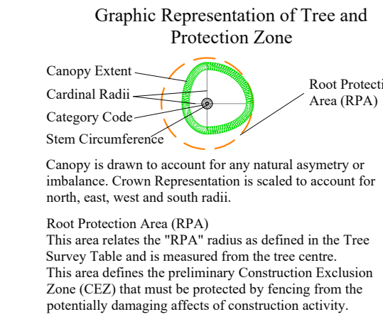
Auburn Tree Protection Plan North East 1/1 _ Scale 1:500 @ A1
